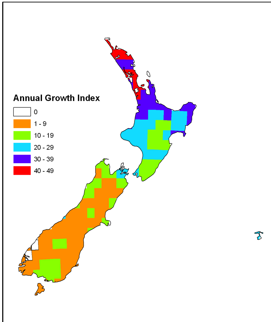
Figure 4: New Zealand showing population growth potential for Puccinia psidii under current (1971-1990) climate averages as indicated by the CLIMEX Annual Growth Index.
