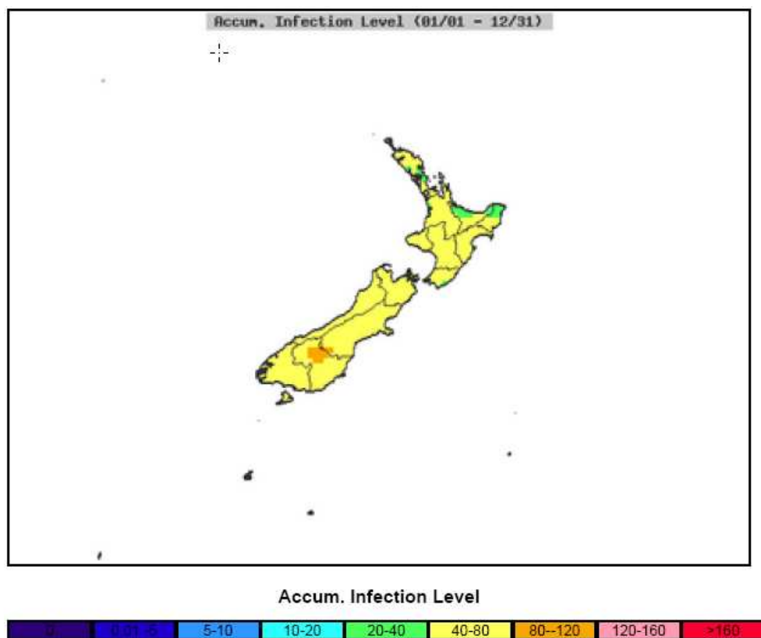
Figure 9: Accumulated infection level for Puccinia psidii in New Zealand modelled using the parameters detailed in Appendix 1.
