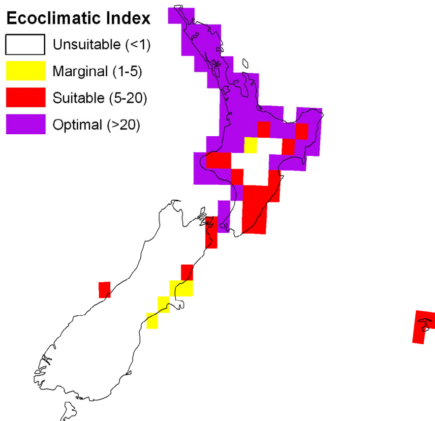
Figure 2: New Zealand showing climate suitability for Puccinia psidii under current (1971-1990) climate averages as indicated by the CLIMEX Ecoclimatic Index. unsuitable ( EI < 1 ); marginal ( 1 < EI < 5 ); suitable ( 5 < EI < 20 ); Optimal ( EI > 20 )
